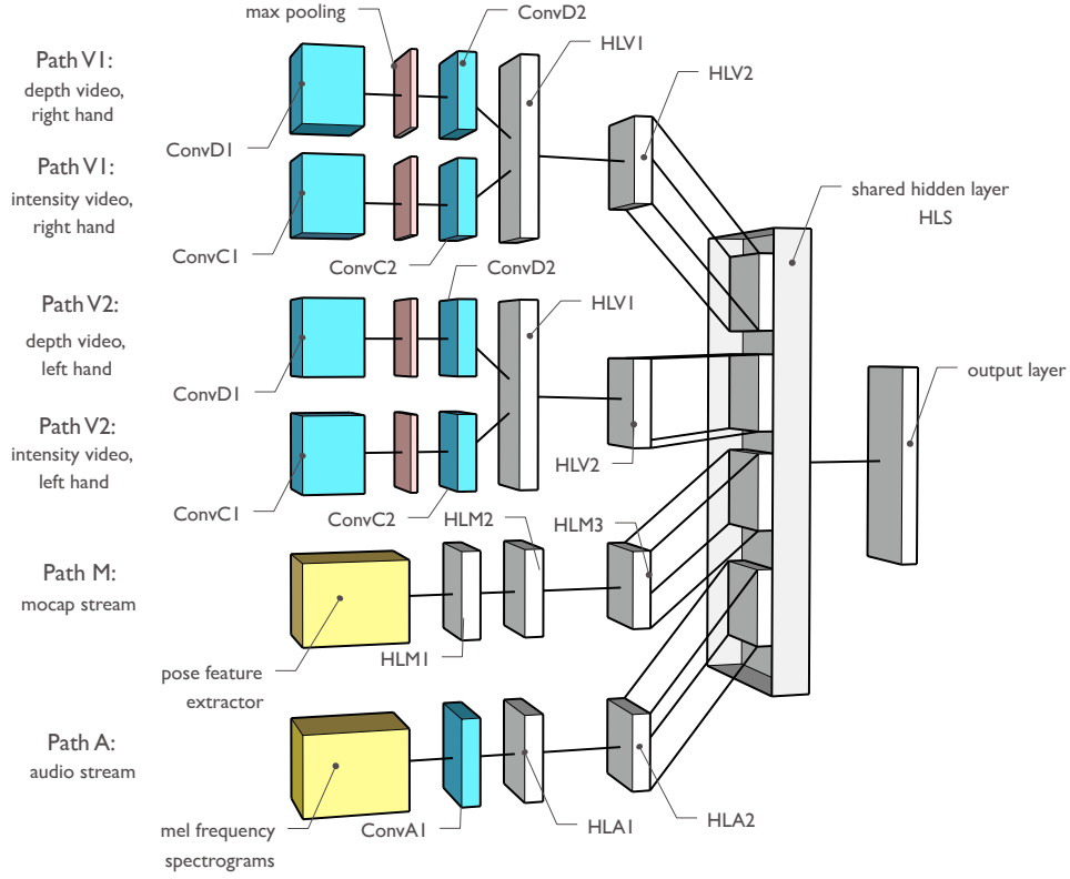
Figure 42 – Single-scale deep architecture. Individual classifiers are pre-trained for each data modality (paths V1, V2, M, A) and then fused using a 2-layer shared fully connected network initialized in a specific way (see Sec. 3.4). The first layers of paths V1 and V2 perform 3D convolutions followed by 3D max pooling eliminating the temporal dimension (not to be confused with V1 and V2 in the human visual system). The second layers on these paths are exclusively spatial. Weights are shared across the V1 and V2 paths.
