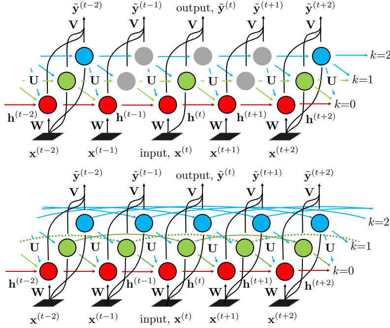
Figure 74 – Comparison of the original Clockwork RNN, proposed by Koutnik et al. [161], and its modification called Dense Clockwork RNN, proposed in this work.
