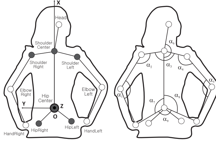
Figure 43 – The proposed pose descriptor is calculated from normalized coordinates of 11 upper body joints, also including their velocities and accelerations, three sets of angles (triples of joints forming inclination angles are shown on the right) and pairwise distances. The body coordinate system (shown on the left) is calculated from 6 torso joints (shown in dark gray on the left).
