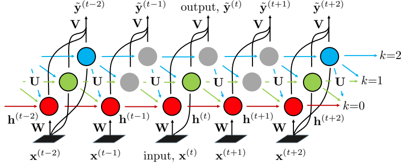
Figure 26 – An example of a Clockwork Recurrent Neural Network (CWRNN) [161] with 3 temporal bands, exponential low and a base of 2. Increasing k indicates lower operating frequency. Grey color indicates inactivity of a slow unit (during both training and test time) at a given iteration t , meaning that the value from the last time when it was active is propagated.
