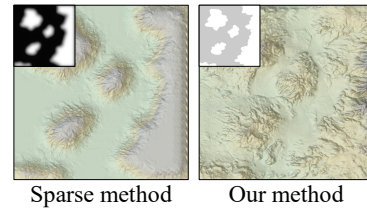
Fig. 20. Comparison between the sparse method from [Guérin et al. 2016] and our levelset synthesizer. Our method produces a vast variety of land-forms features whereas sparse modeling reproduces similar details.
