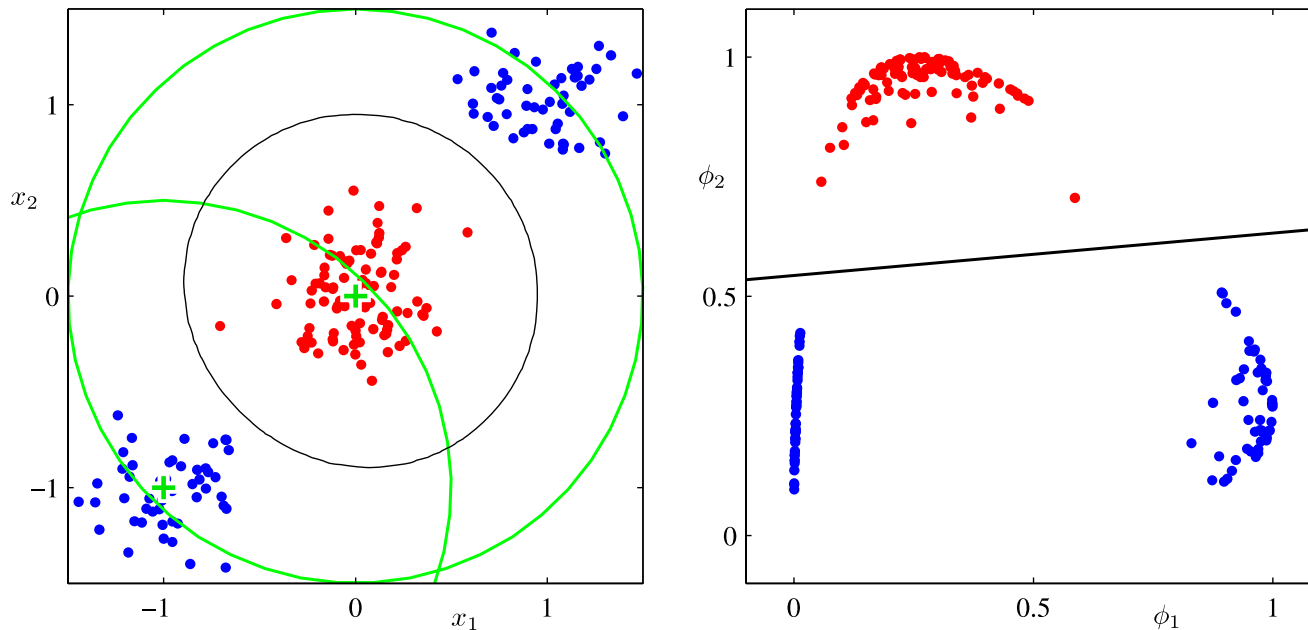
Gaussian basis functions
